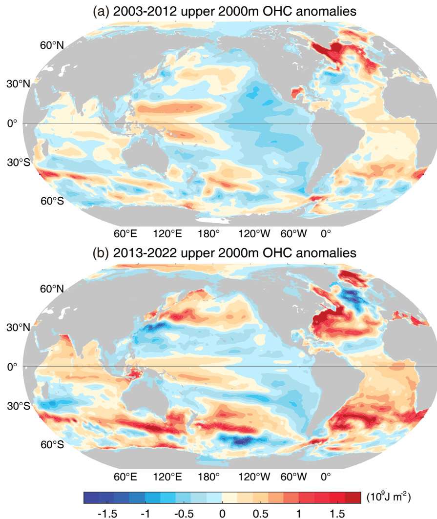
Fig. 6. Anomalies of upper 2000 m OHC from (a) 2003 to 2012 and (b) 2013 to 2022, relative to a 1981–2010 baseline but with the global mean value removed for each map [data updated from Cheng et al. (2017a)].
