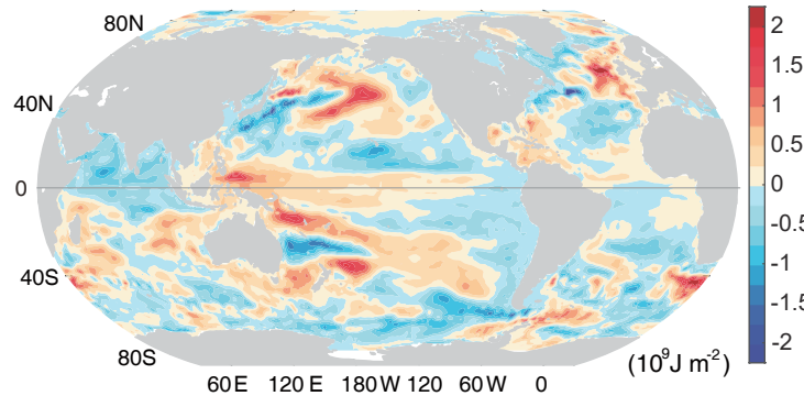
(c) 2022 OHC (0-2000m) anomaly relative to 2021 (NCEI/NOAA)
